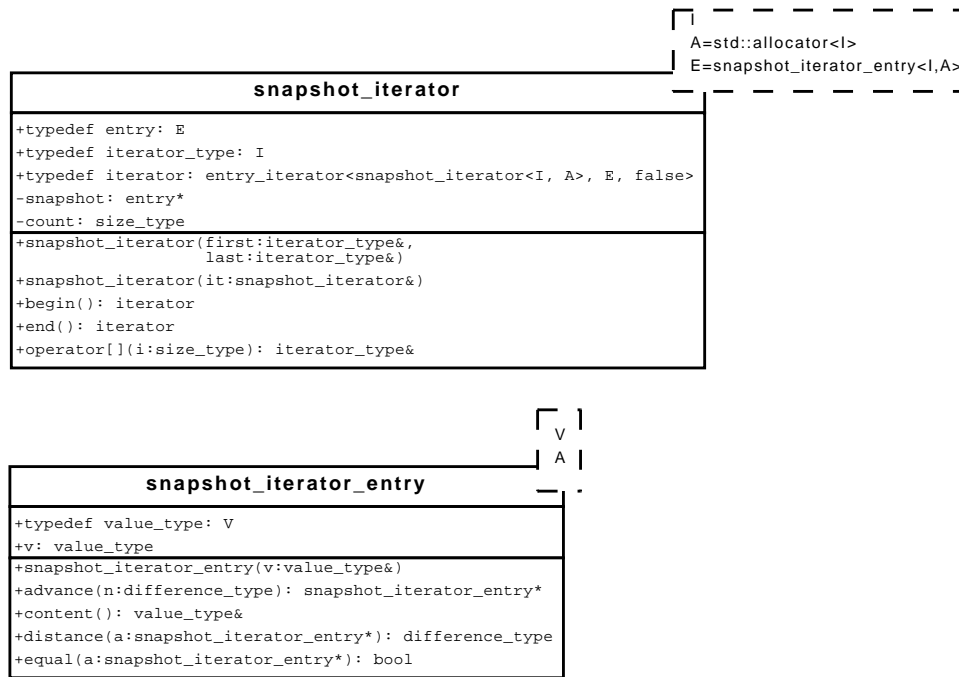
Figure 4. An overview of the snapshot iterator design
